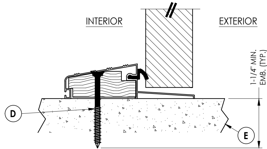
3 3 VERTICAL CROSS SECTION Outswing Sill
