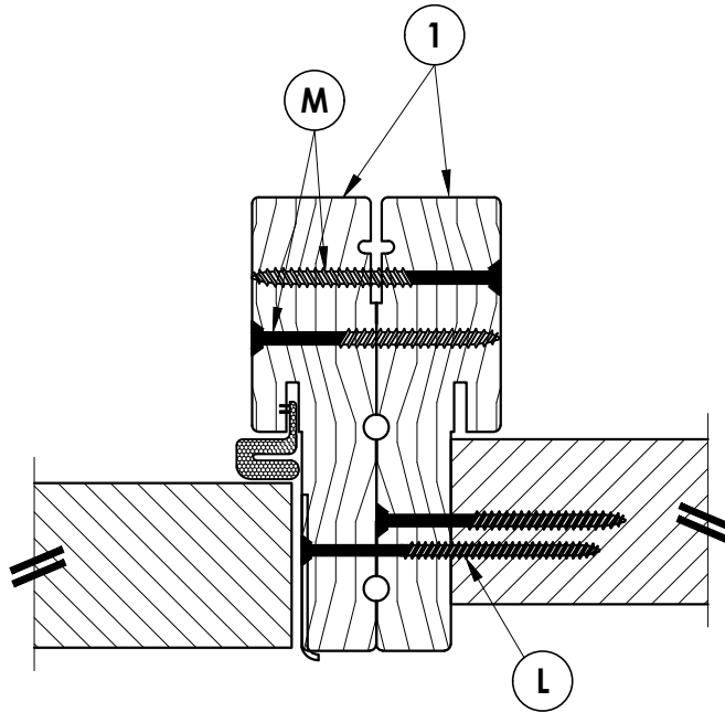
6 HORIZONTAL CROSS SECTION 2 @ BACK-TO-BACK JAMBS
